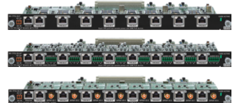
MX-TPS2-IB-P, -AP, -SP Part No: 9112 0035 (P), 9112 0036 (AP), 9112 0037 (SP) TPS input board with PoE option.
